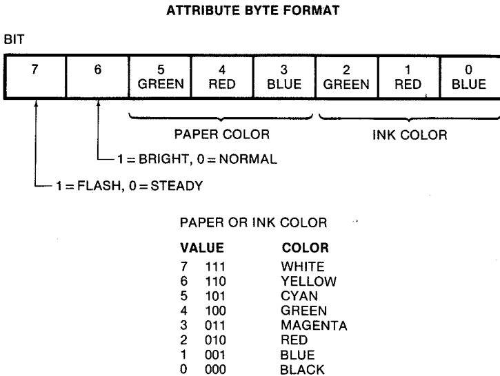
Fig. 8-6. Attribute byte structure. (Courtesy Timex Computer Corp.)
